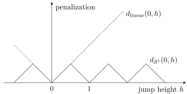
Fig. 1 In contrast to the linear distance ( dashed ), the cyclic distance d_{S^1} ( solid ) accounts for the periodicity of S^1
