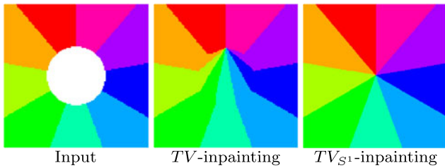
Fig. 8 Inpainting of periodic hue values. While total variation regularization ( center ) does not handle wrap-arounds correctly (shrinking the interface with the highest value jump, here from magenta to red ) the proposed TV_{S^1} formulation ( right ) is designed to provide an optimal solution for cyclic structures at no additional cost (Color figure online)
