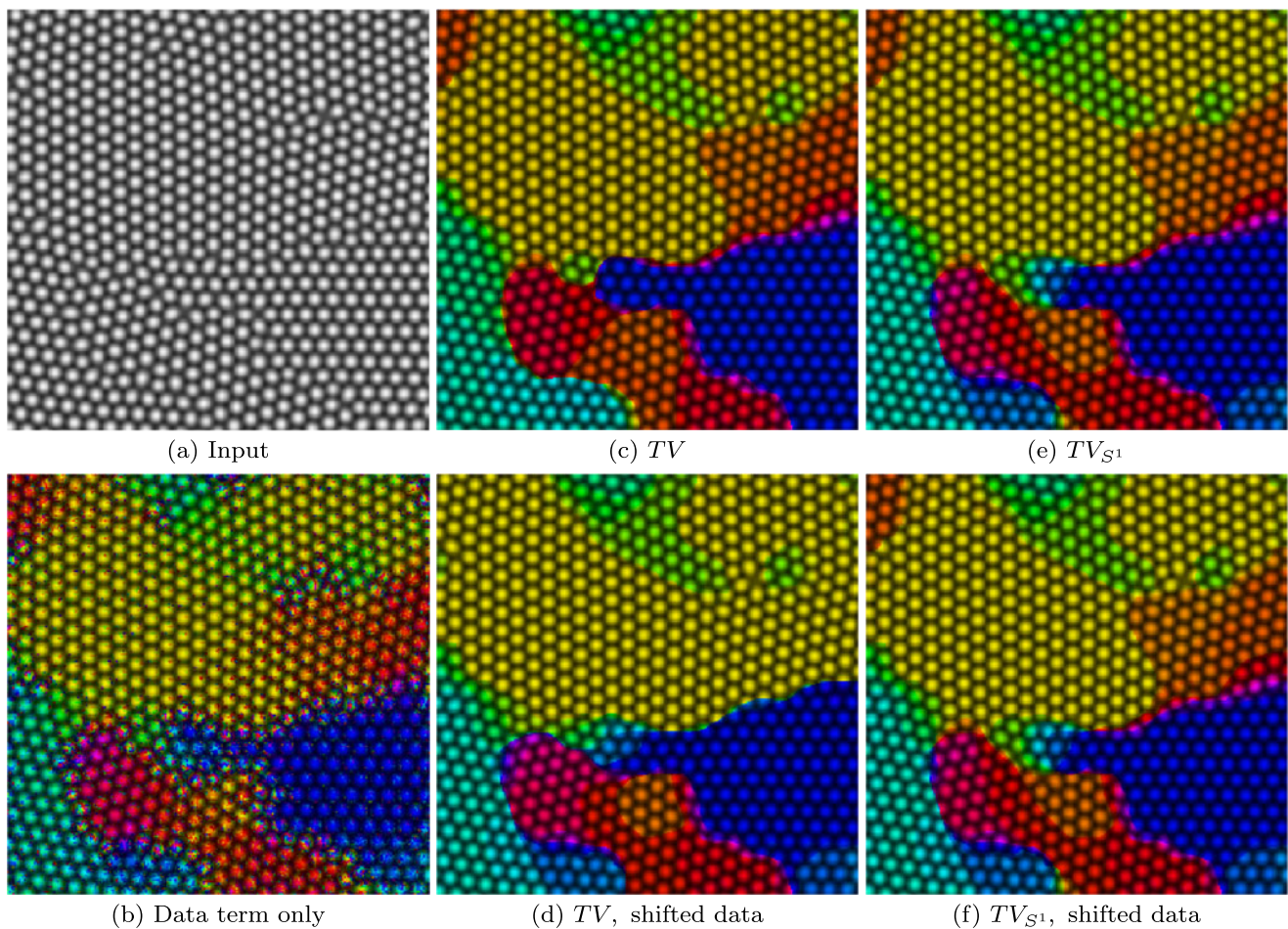
Fig. 10 Segmentation of regions with homogeneous atom lattice orientation , coloring different orientations by different hues. This example demonstrates the cyclic shift invariance of TV_{S^1} in Proposition 5. The results in (e) for the original data term \varrho(x, t) and in (f) for the
