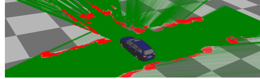
Fig. 12. Occupancy grid for a typical parking lot scene after vehicle has passed several occupied spaces and positioned itself in front of an empty one.
