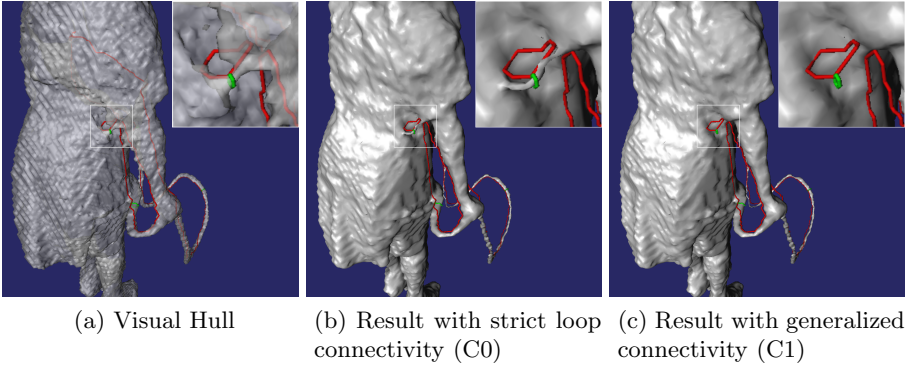
Fig. 3: (a) In some cases artifacts of the visual hull can lead to spurious handle loops which should not be preserved in the final reconstruction. (b) The constraint C0 strictly preserves all loops in the solution. (c) Relaxing the topology preserving constraint to our generalized connectivity constraint allows to suppress handles where the photoconsistency is not strong enough. The rope, where the support of the photoconsistency is sufficient, is still completely preserved. Handle and tunnel loops are depicted in green and red, respectively.
