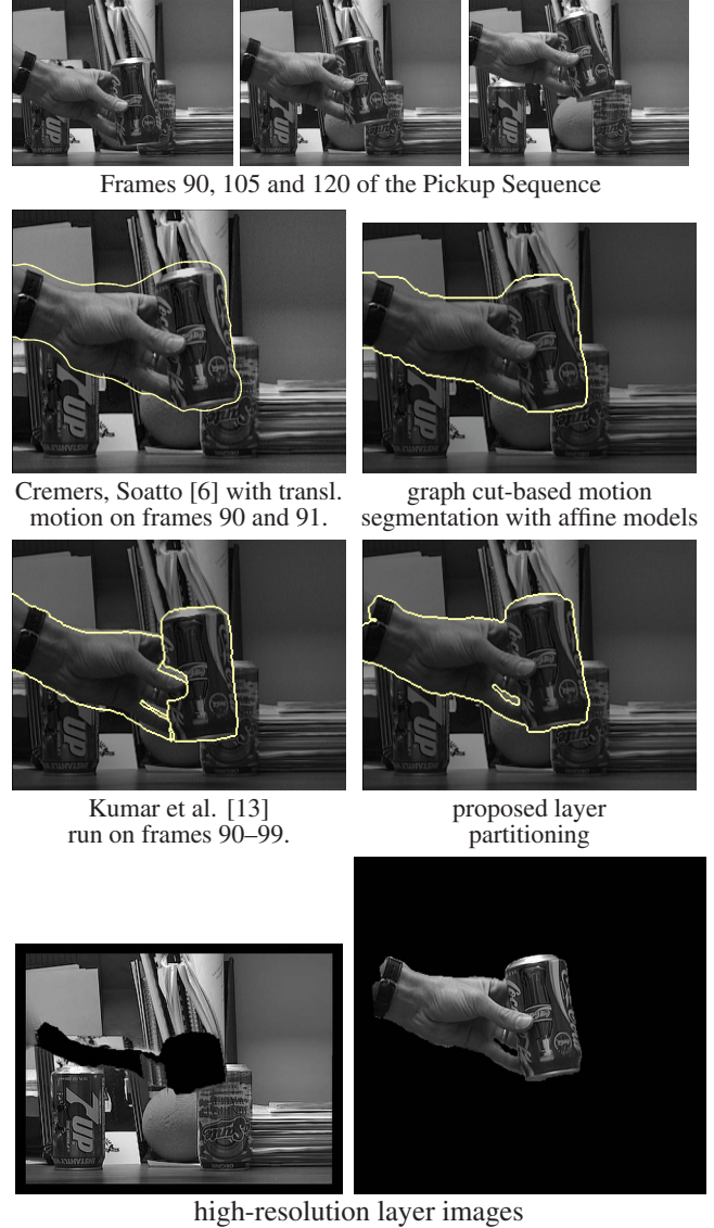
Figure 3. Comparison on the Pickup Sequence: With the proposed method, the tightest boundaries are obtained.
